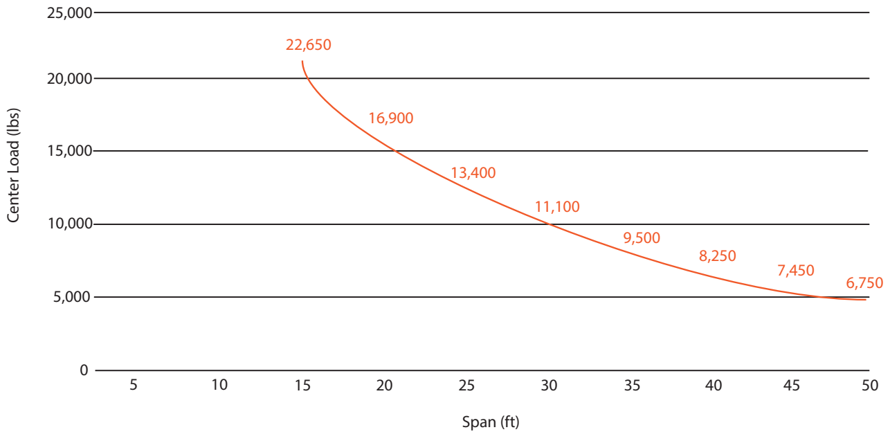
Modulus-X™ Mx|99| 9x18 Center Load Test
